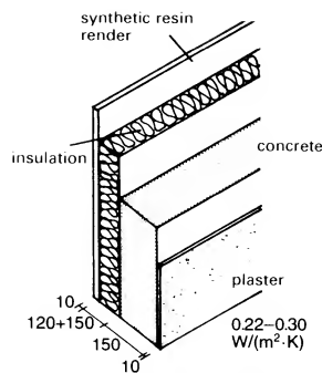
② Concrete with bonded insulation panels 0.22-0.30 W/(m 2 ·K)
